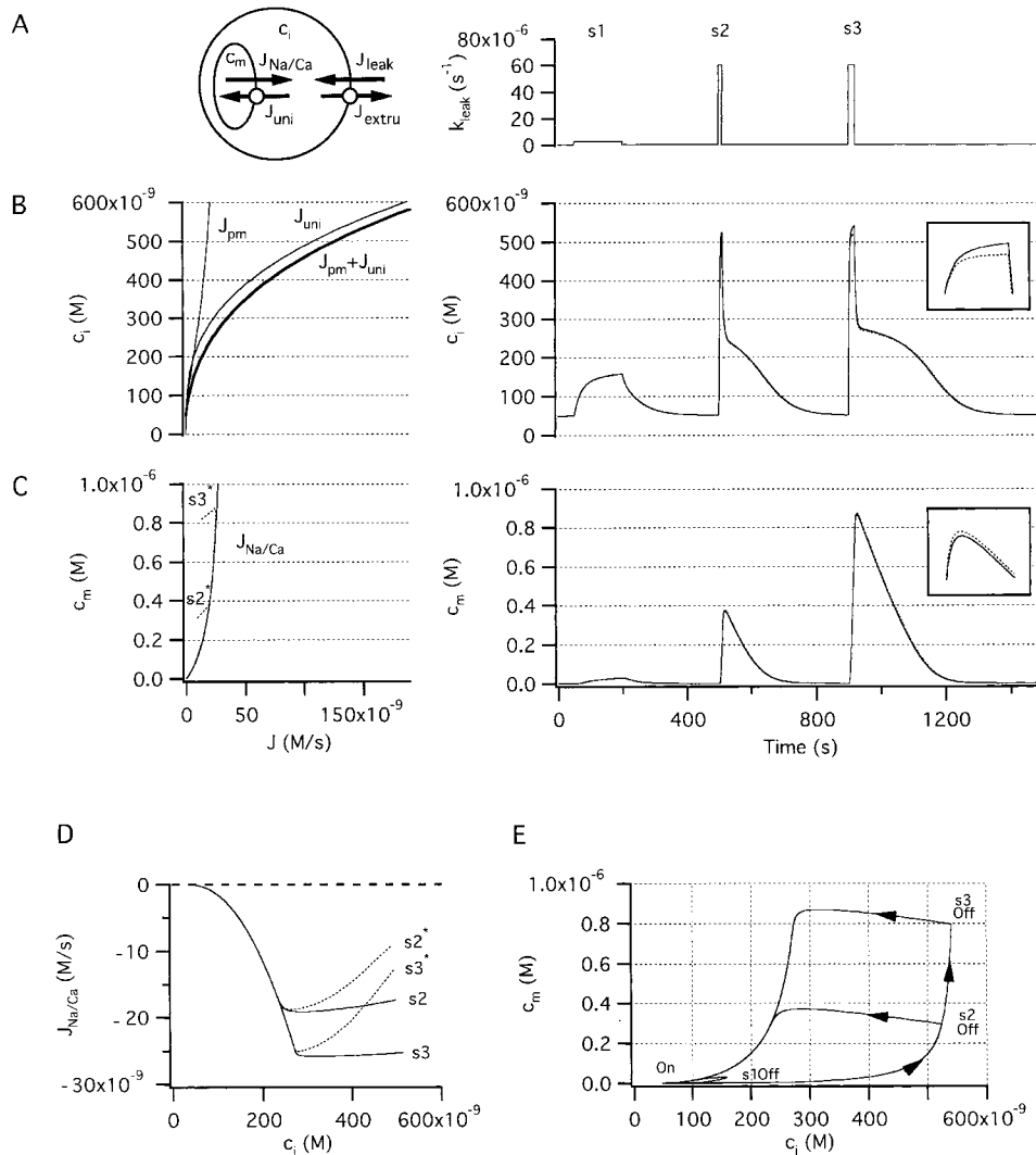
Figure 3. Simulated changes in cytosolic and mitochondrial \text{Ca}^{2+} concentration during and after stimulated Ca entry. (A, left) Schematic of the model used in the simulations indicating compartments (with \text{Ca}^{2+} concentration c_i and c_m ) and pathways for \text{Ca}^{2+} movement between compartments. The net plasma membrane \text{Ca}^{2+} flux, J_{\text{pm}} is the sum of J_{\text{leak}} and J_{\text{extru}} and the net mitochondrial \text{Ca}^{2+} flux is the sum of J_{\text{uni}} and J_{\text{Na/Ca}} . (Right) \text{Ca}^{2+} entry was stimulated by increasing the plasma membrane leak rate constant ( k_{\text{leak}} ). (B, left) c_i -dependent components of the total \text{Ca}^{2+} flux: J_{\text{pm}} , J_{\text{uni}} and J_{\text{pm}} + J_{\text{uni}} . Note that J_{\text{pm}} is calculated using the basal \text{Ca}^{2+} entry rate constant and therefore does not apply during stimulation. (Right) Simulated changes in c_i during and after each stimulus. Solid curves show simulated c_i values in the case where J_{\text{Na/Ca}} depends only on c_m (Eq. 17), dotted curves illustrate the case where J_{\text{Na/Ca}} depends on both c_m and c_i (Eq. 19). Inset shows on an expanded scale the small effect of including the c_i -dependent inhibitory factor in the definition of J_{\text{Na/Ca}} ; inset represents a 100 nM range of c_i around the peak of the response to stimulus s3. (C, left) J_{\text{Na/Ca}} and its dependence on c_m according to Eq. 17 (solid trace) or on c_m and c_i according to Eq.
