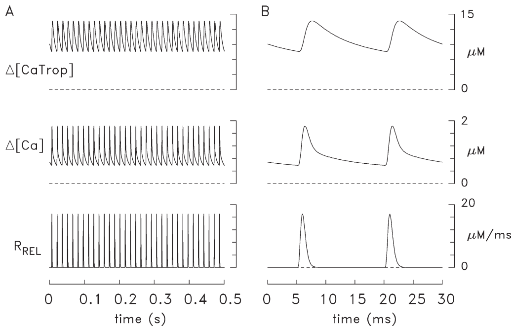
Figure 6. Simulation results when the midshipman model is driven to steady state with the Ca^{2+} release waveform defined by Eq. 3 repeated at 67 Hz. The values of R , \tau_1 , and \tau_2 in Eq. 3 were 2,008 \mu M/ms , 0.8 ms, and 0.32 ms, respectively. The simulated traces are R_{REL} (bottom), \Delta[Ca^{2+}] (middle), and \Delta[CaTrop] (top); the results for \Delta[CaATP] , \Delta[CaParv] , \Delta[CaPump] , and \Delta[CaPumped] (not depicted) are described in the text (see Simulation of myoplasmic Ca^{2+} movements during long-lasting high-frequency stimulation and Simulations with a more-sensitive Ca^{2+} pumping-pCa relation in Results). (A and B) In A, the traces are shown on a time base like that on the right side of Fig. 5; in B, two cycles of the traces on the left side are shown on an expanded time base.
