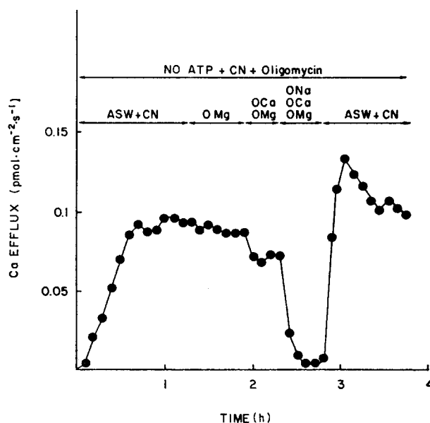
FIGURE 9. The effect of external magnesium, calcium, and sodium on the calcium efflux in the absence of internal ATP. Abscissa: time in hours. Ordinate: calcium efflux in \text{pmol} \cdot \text{cm}^{-2} \cdot \text{s}^{-1} . [\text{Ca}]_i = 0.3 \mu\text{M} . T^\circ = 22^\circ\text{C} . Axon diameter: 400 \mu\text{m} .
