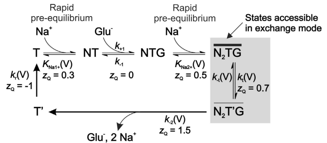
Scheme 1. Pseudo four-state model used for kinetic modeling of EAAT4 anion currents. The detailed kinetic parameters used for modeling are listed in table 1.
